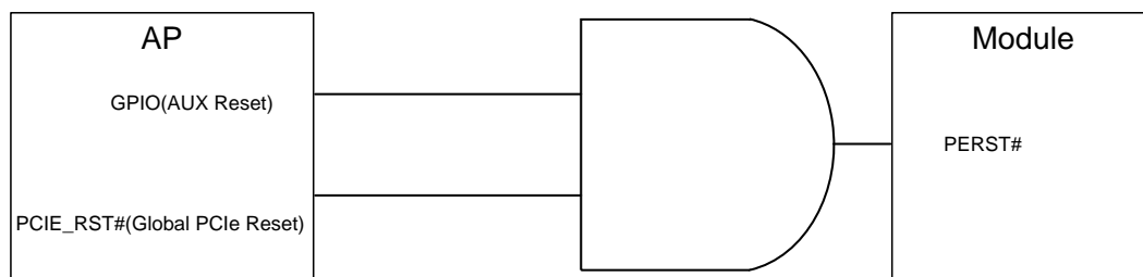
Figure 10: Reference Circuit for Laptop PCIe Reset Logic
