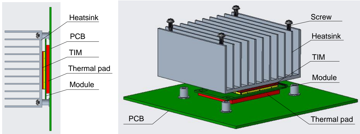
Figure 40: Placement and Fixing of the Heatsink
