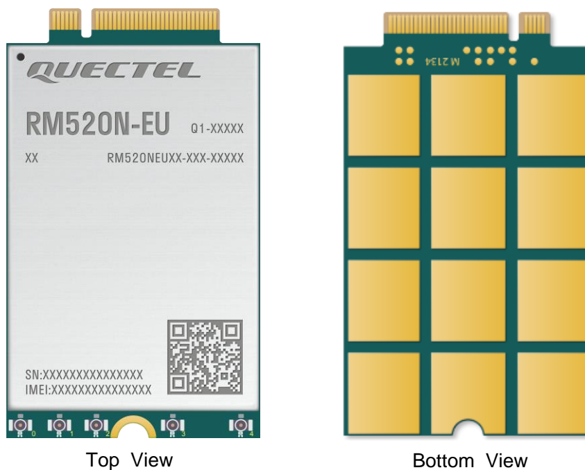
Figure 44: Top and Bottom Views of the RM520N-EU
