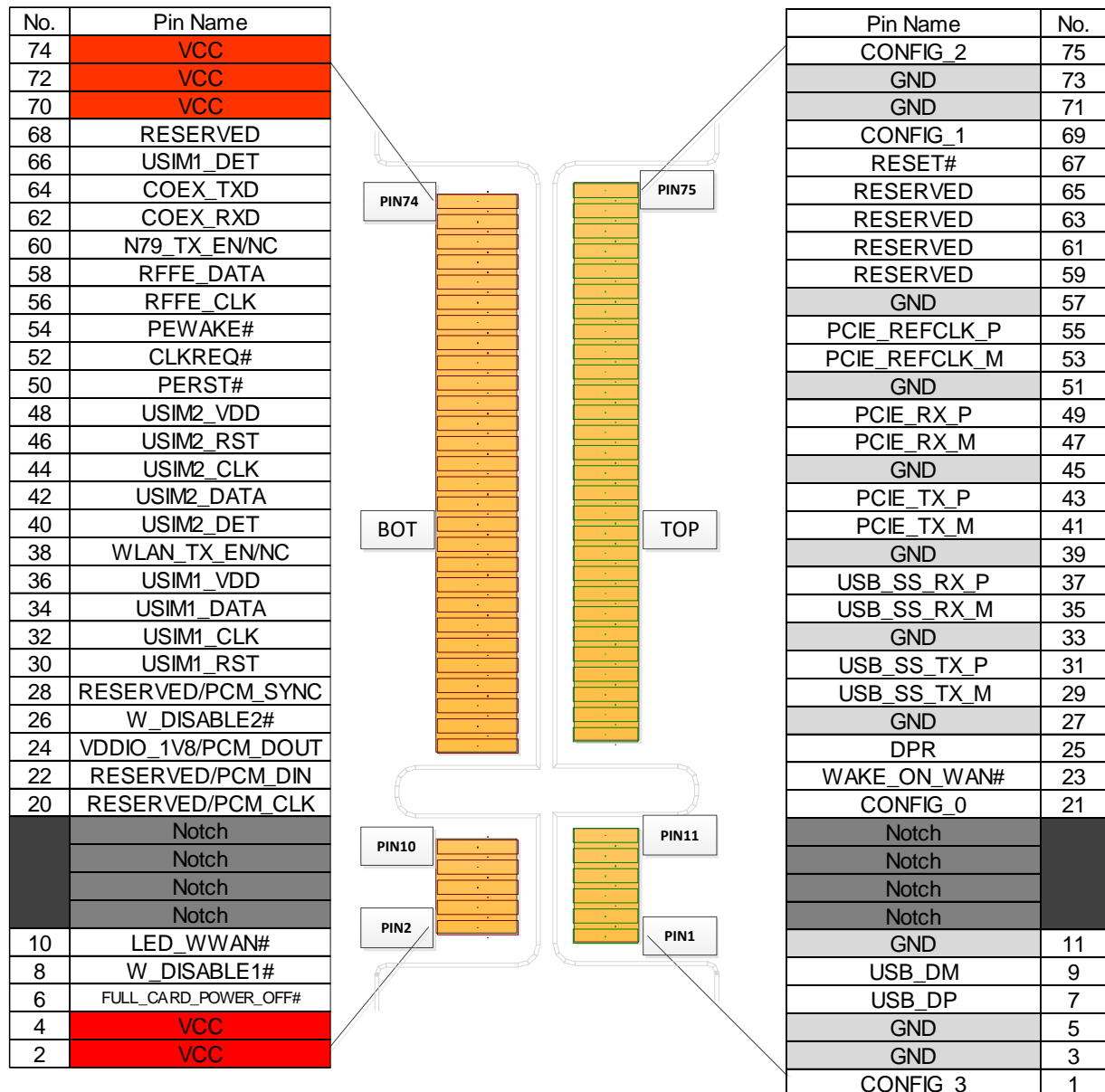
Figure 2: Pin Assignment 8
