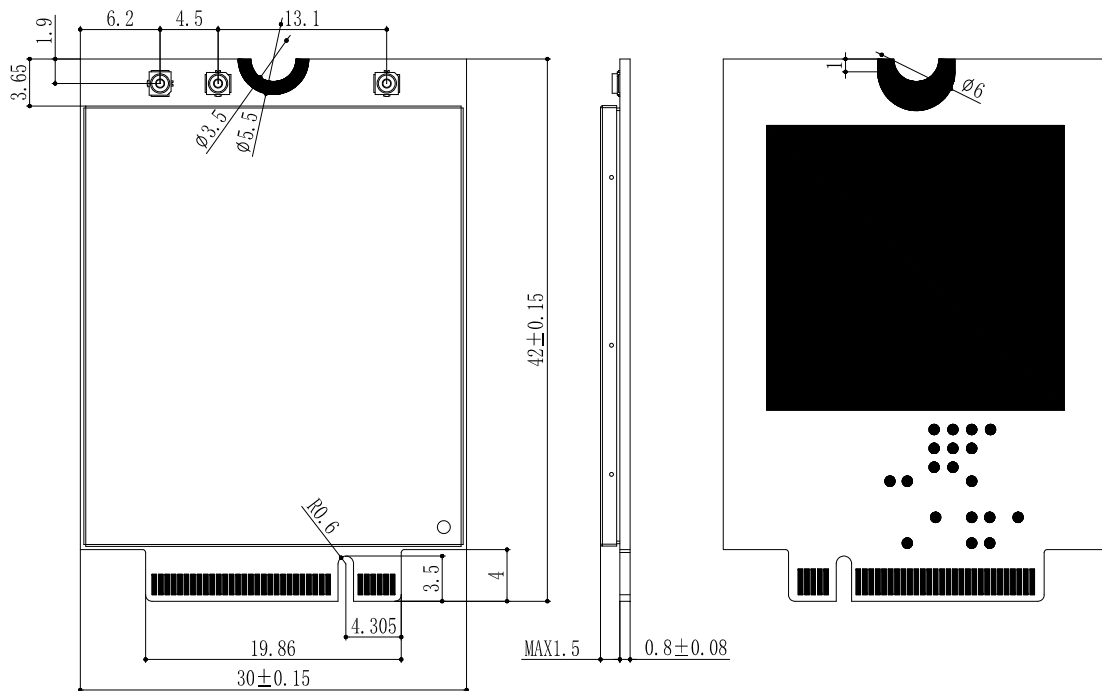
Figure 34: Mechanical Dimensions of EM12-G (Unit: mm)
