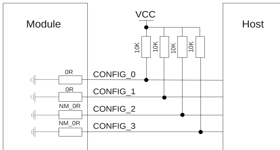
Figure 27: Reference Circuit of Configuration Pins
