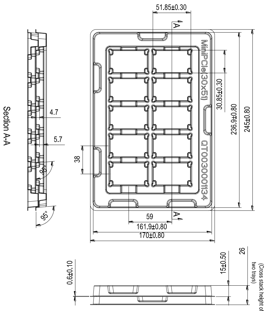
Figure 39: Blister Tray Dimension Drawing
