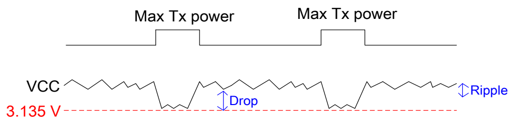
Figure 5: Power Supply Limits during Radio Transmission
