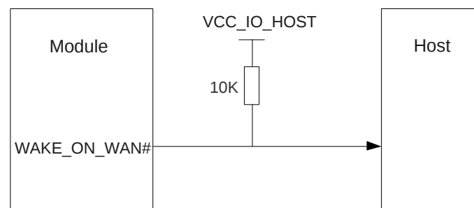
Figure 26: Reference Circuit of WAKE_ON_WAN#
