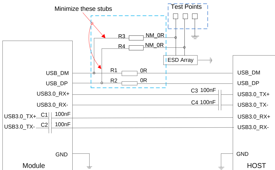
Figure 18: Reference Circuit of USB 2.0 & 3.0 Interface
