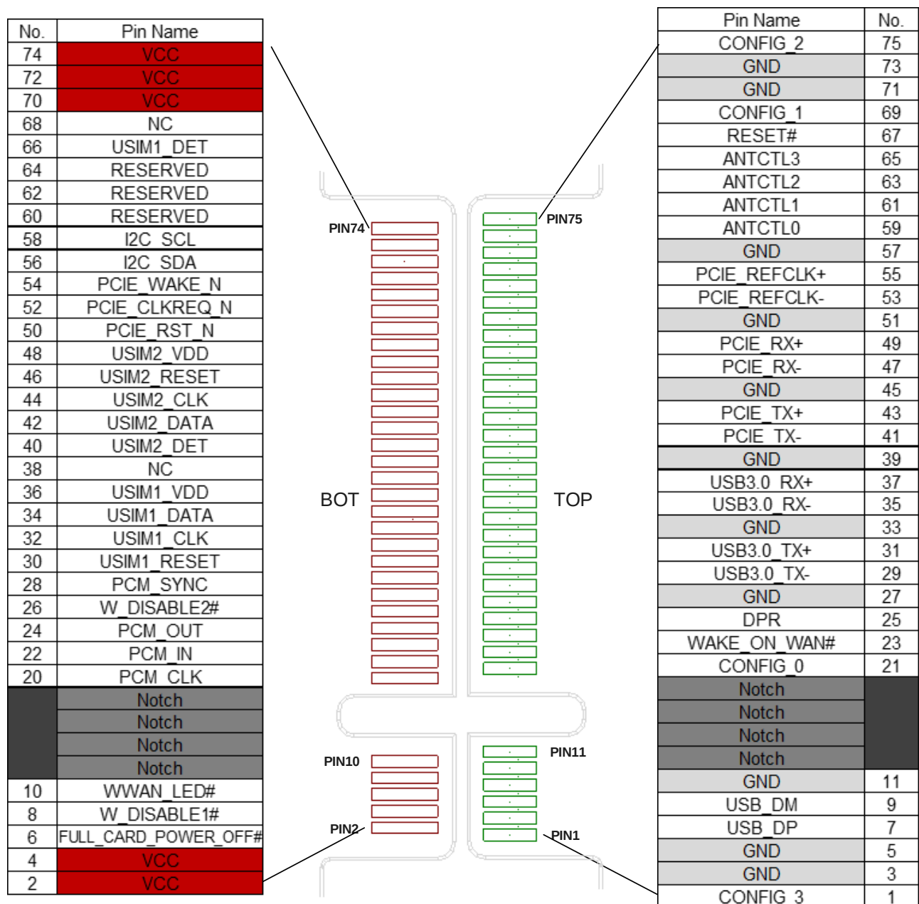
Figure 2: Pin Assignment
