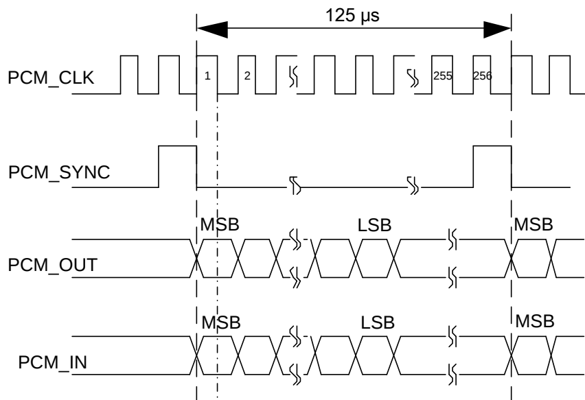
Figure 20: Primary Mode Timing
