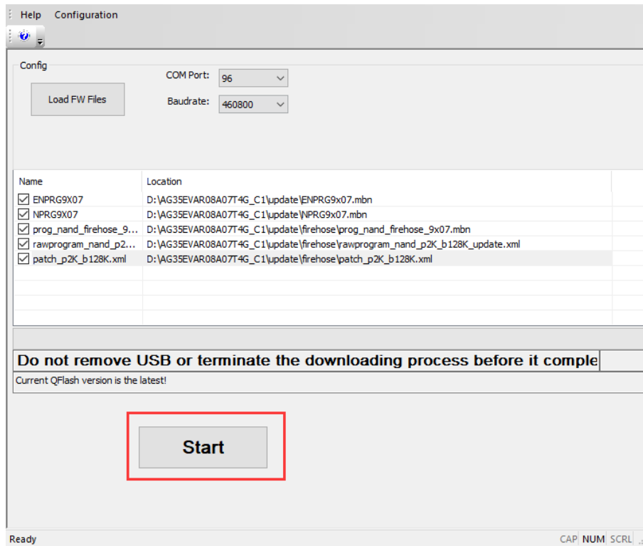
Figure 28: “Start” Button
