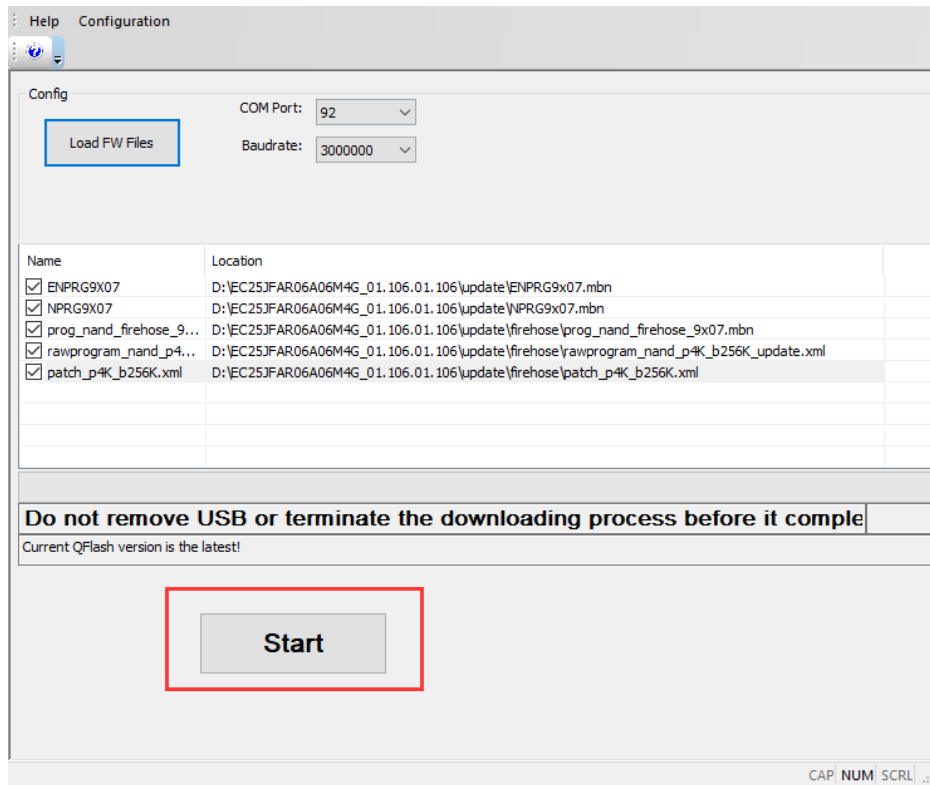
Figure 21: “Start” Button
