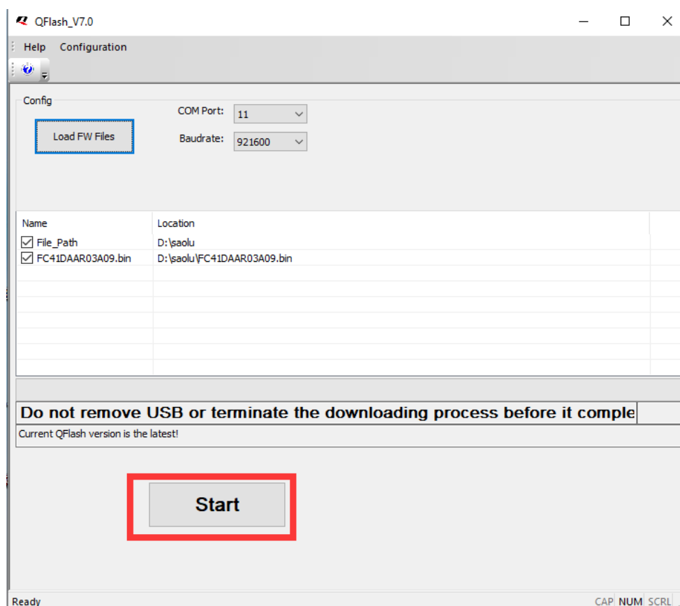
Figure 61: “Start” Button
