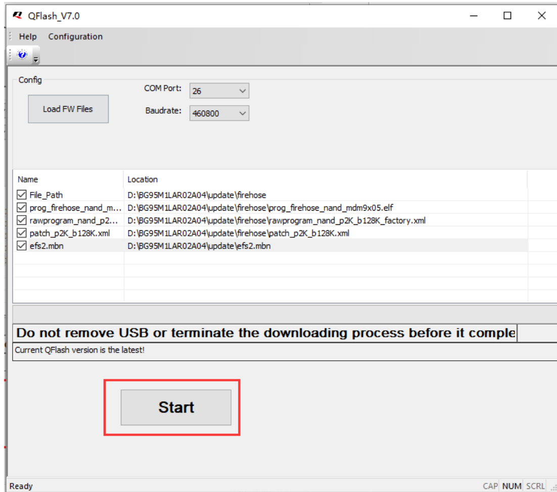
Figure 43: “Start” Button
