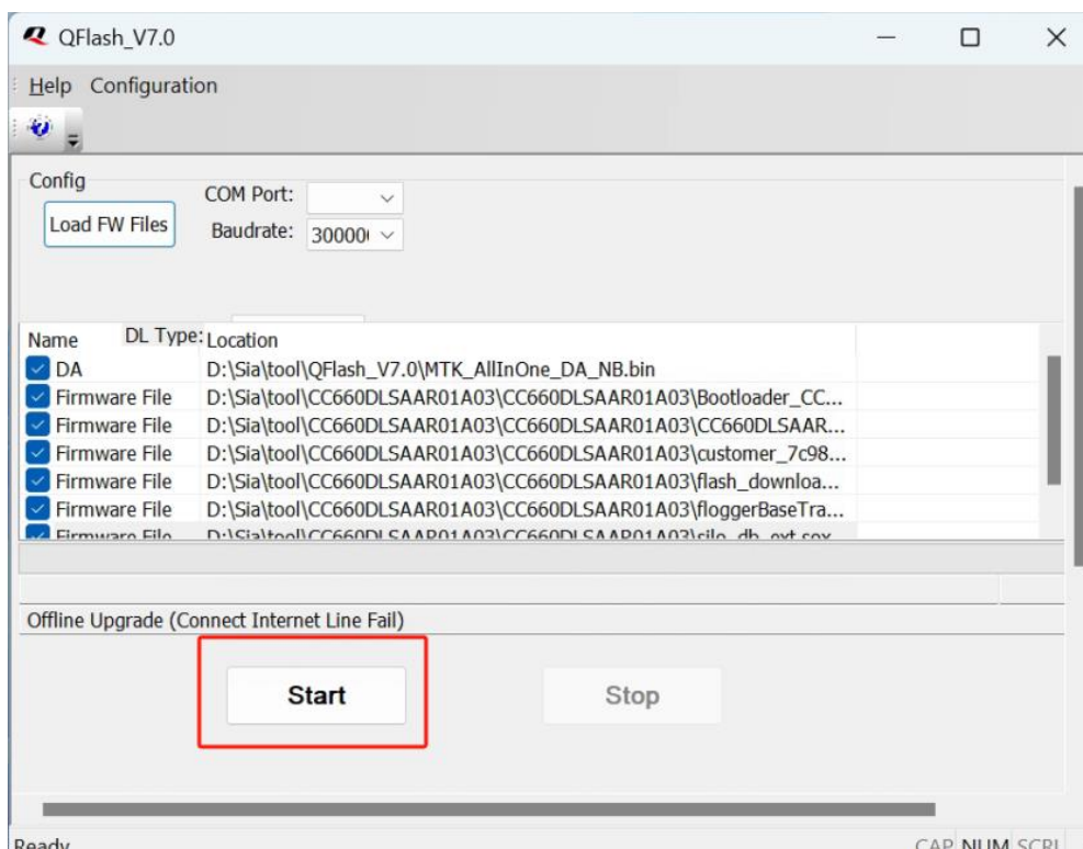
Figure 68: “Start” Button
