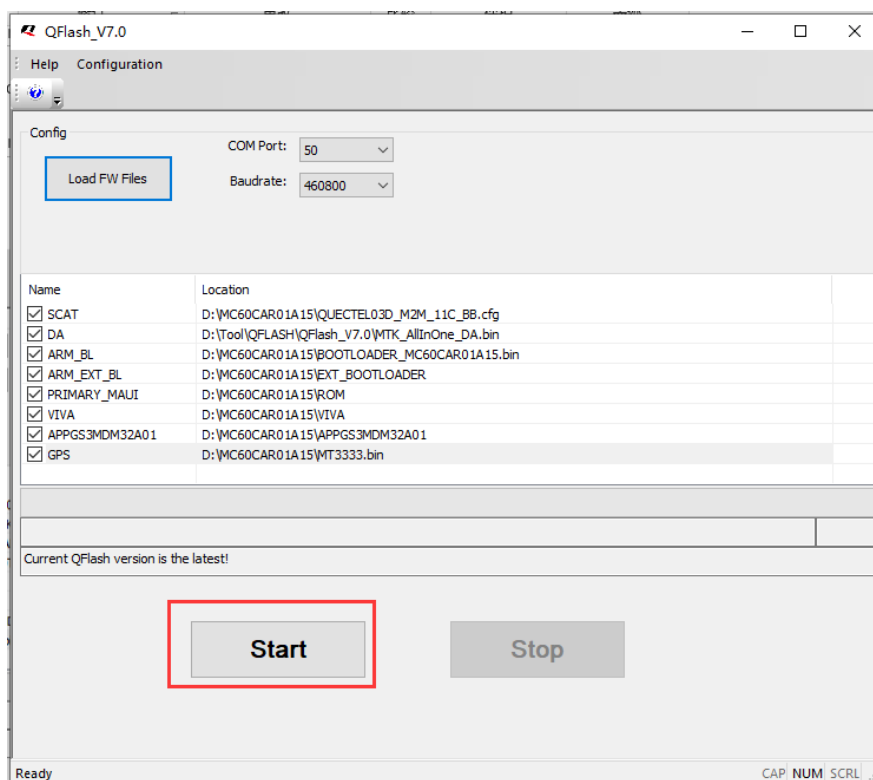
Figure 54: “Start” Button
