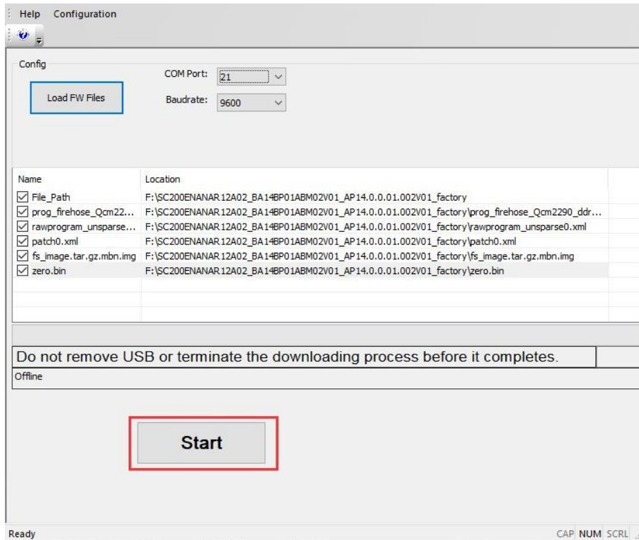
Figure 35: “Start” Button
